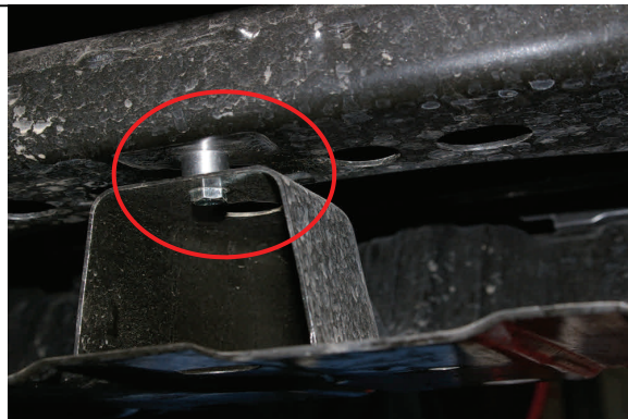
Install (2) skid plate spacers with new hardware
